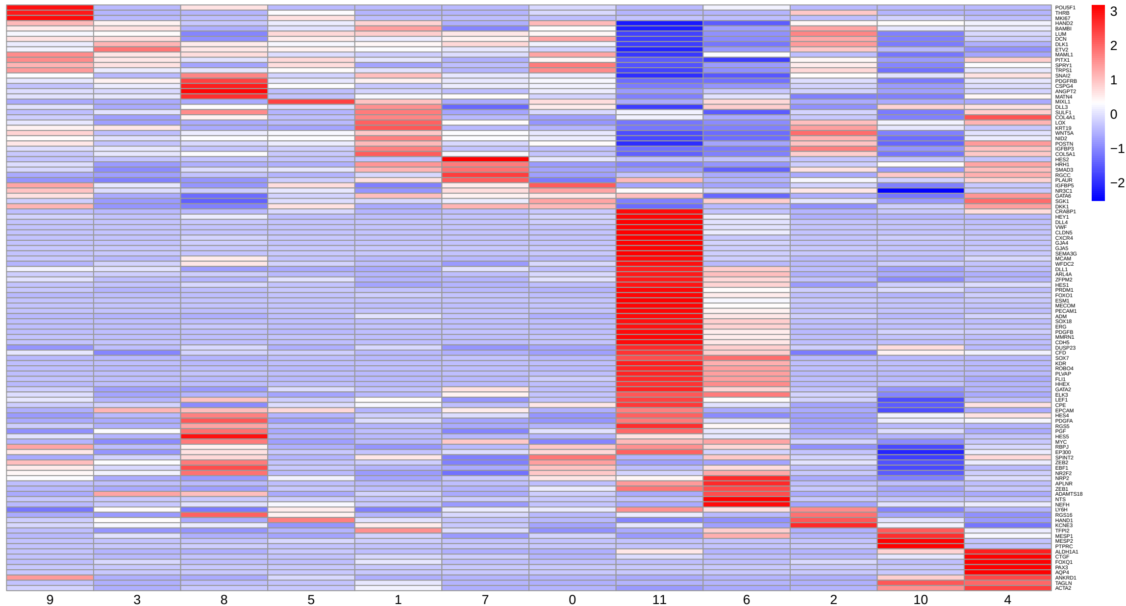
Z-scored gene expression per cluster (RNA assay)
