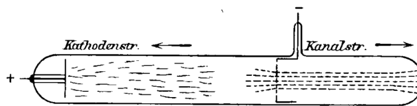
Figure 2: Discharge tube producing cathode rays and canal rays (Stark 1906, 405)
