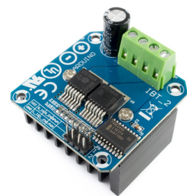
(c) BTS7960
