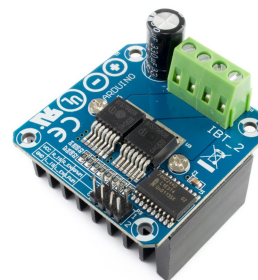
(c) BTS7960
