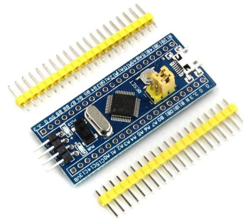
(c) STM32F103C8T6
