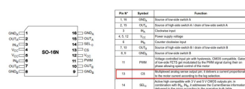
(a) VN7070BAS
