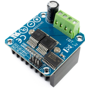
(c) BTS7960
