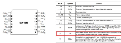
(a) VN7070BAS
