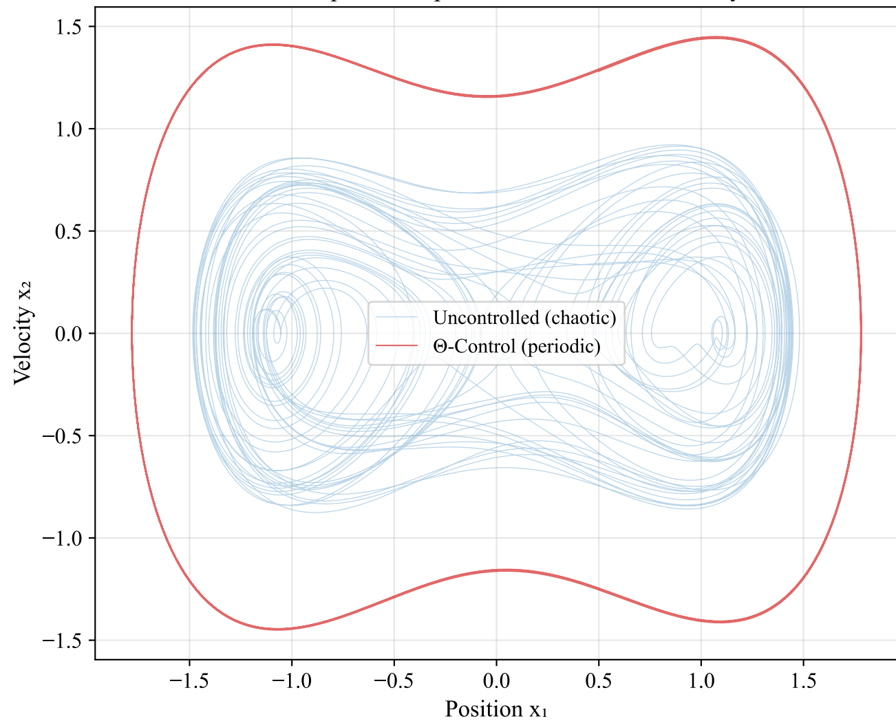
Phase Space Comparison: Chaos vs. Periodicity
