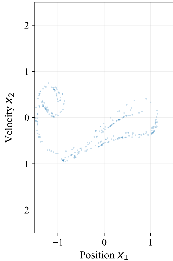
(a) Poincaré Map - Uncontrolled (286 points)
