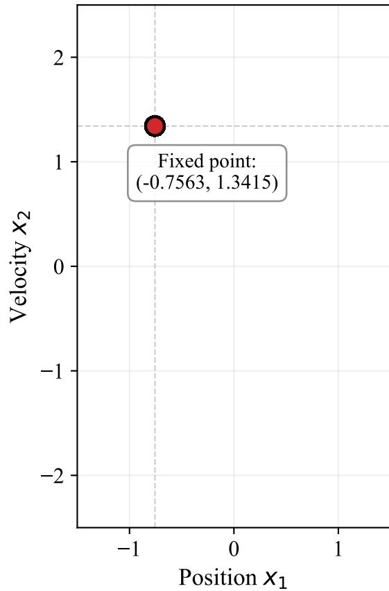
(b) Poincaré Map - \Theta -Control (286 points)
