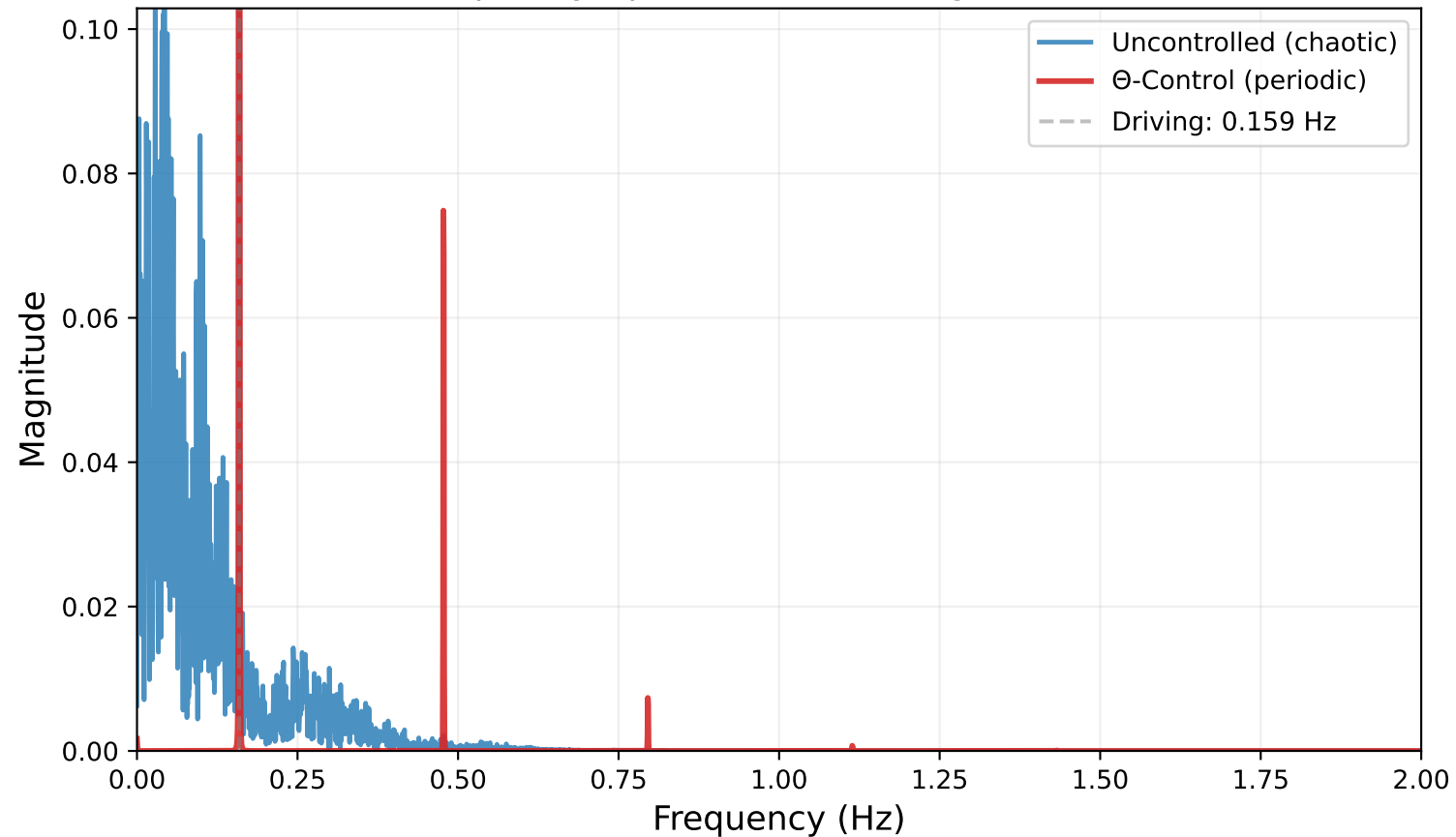
Frequency Spectrum of Duffing Oscillator
