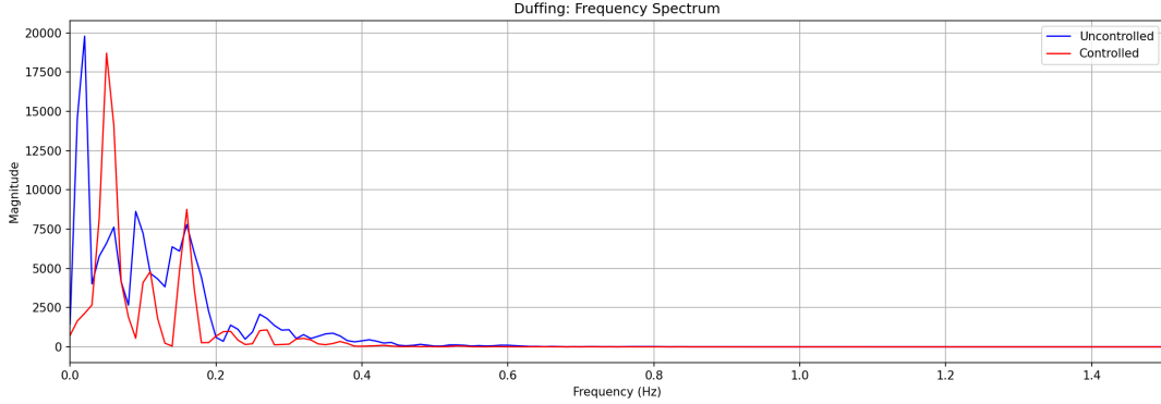
Figure 6: Frequency spectrum of the Duffing response: uncontrolled (blue) shows broad-band chaotic characteristics; controlled (red) shows distinct peaks indicating periodic behavior.
