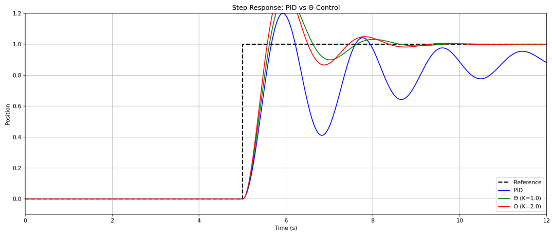
Figure 1: Step response comparison: PID (blue) vs \Theta -Control with K_\theta = 1.0 (green) and K_\theta = 2.0 (red). The reference step occurs at t = 5 s. \Theta -Control achieves it with significantly faster rise time.
