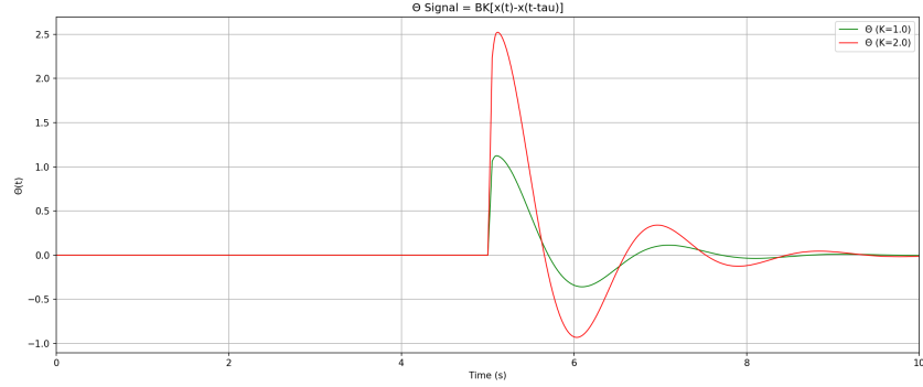
Figure 2: The \Theta signal for different gains. Notice the characteristic oscillatory-convergent behavior, demonstrating how memory actively shapes the control action.
