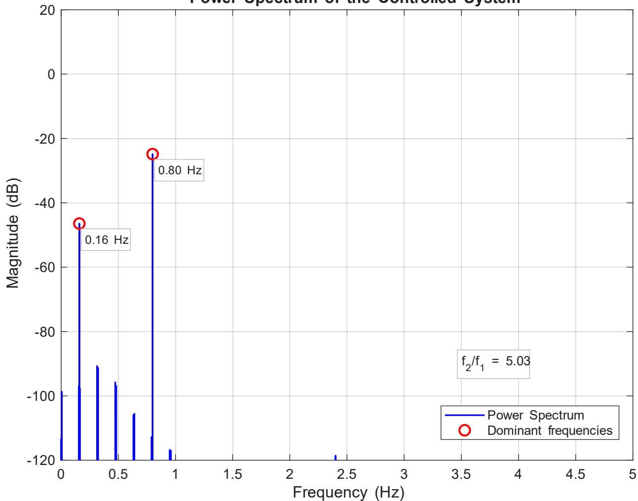
Power Spectrum of the Controlled System
