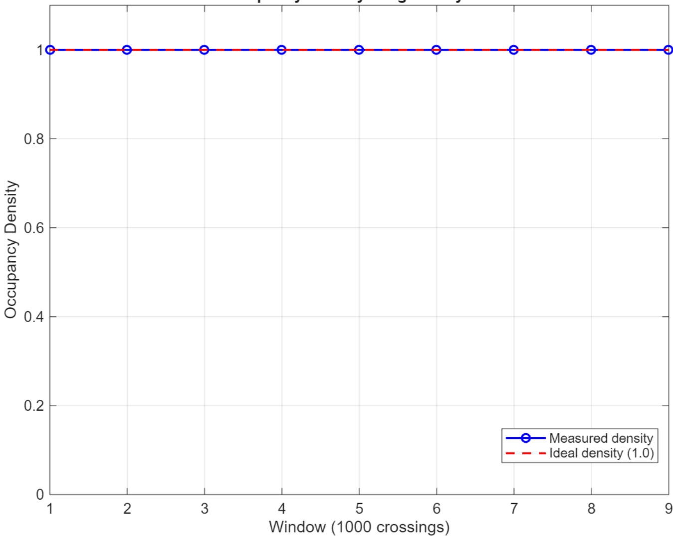
Occupancy Density - Ergodic System
