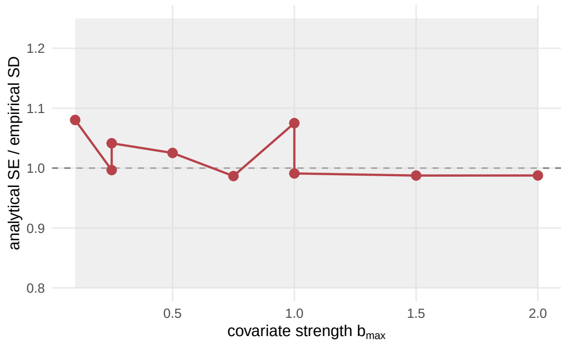
SE calibration vs covariate strength
