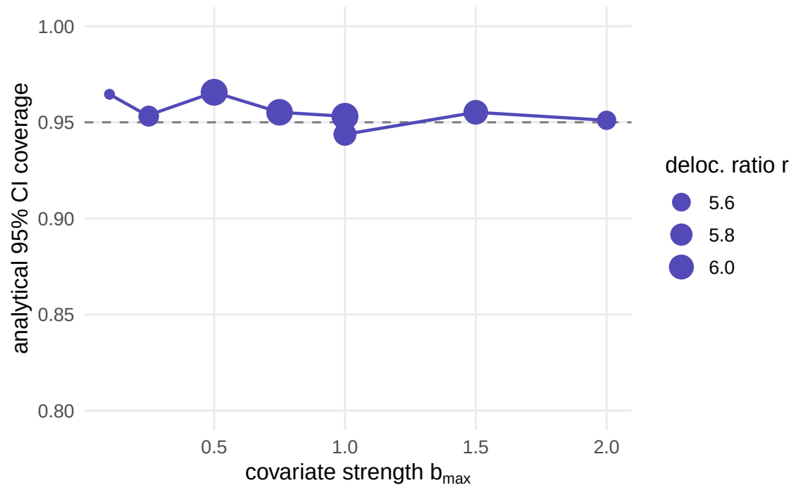
Coverage vs covariate strength (crossover)
