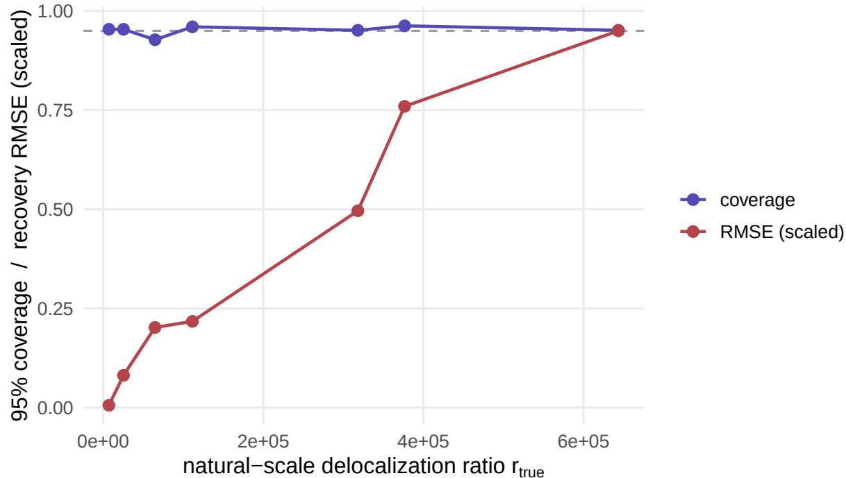
Delocalization crossover (Proposition 16)
