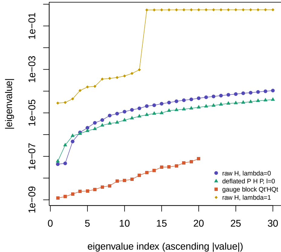
Spectrum tail at eta* — strong (rep 1)
