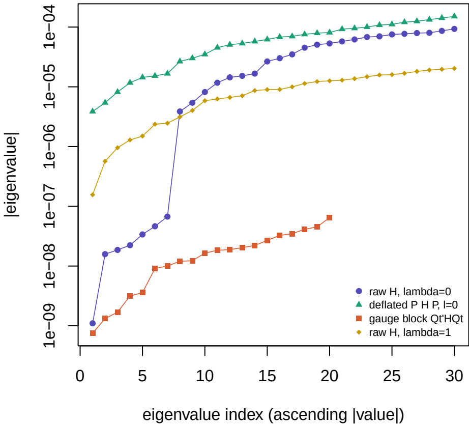
Spectrum tail at eta* — weak (rep 1)
