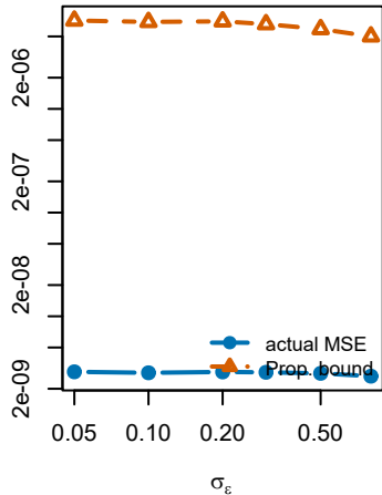
entry-wise MSE
