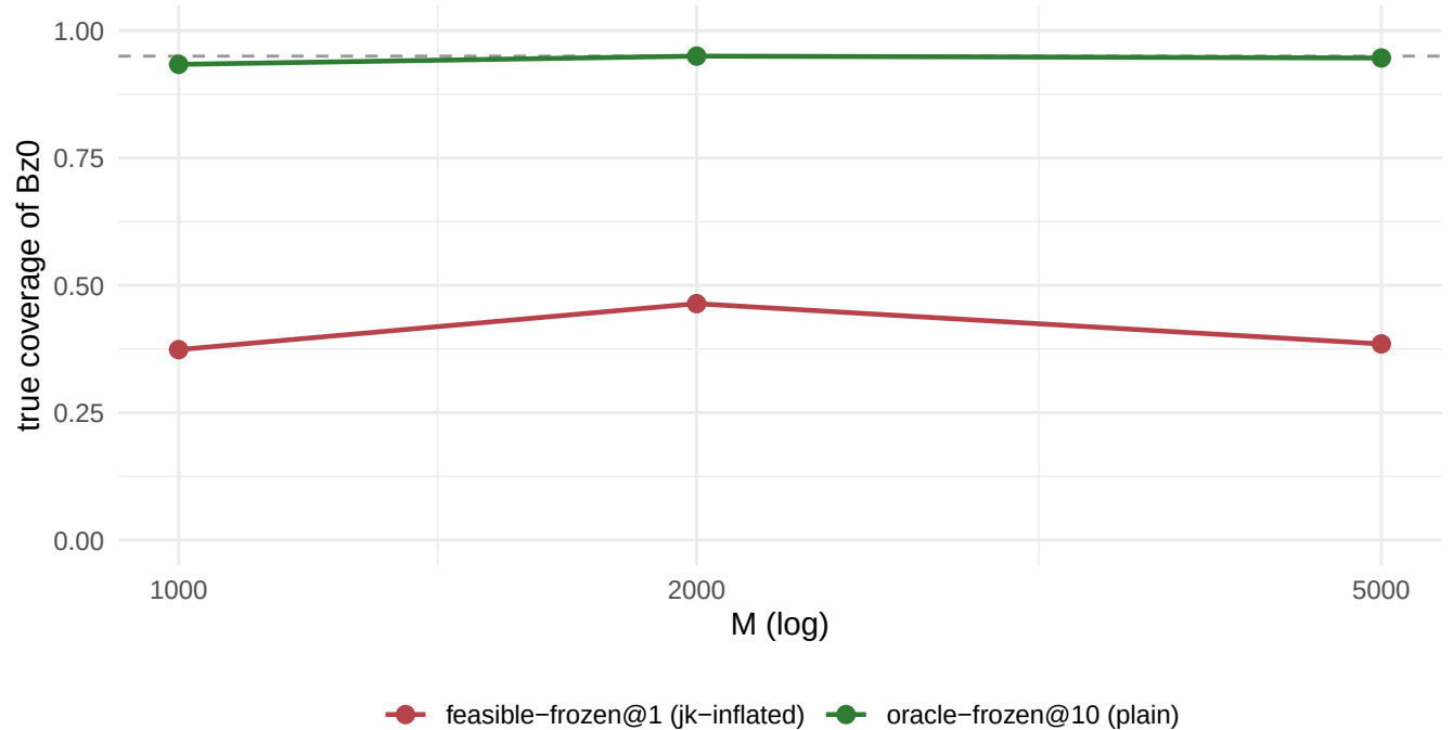
In-regime ( L=1e4 ) coverage: oracle nominal, feasible blocked by anchor variance
