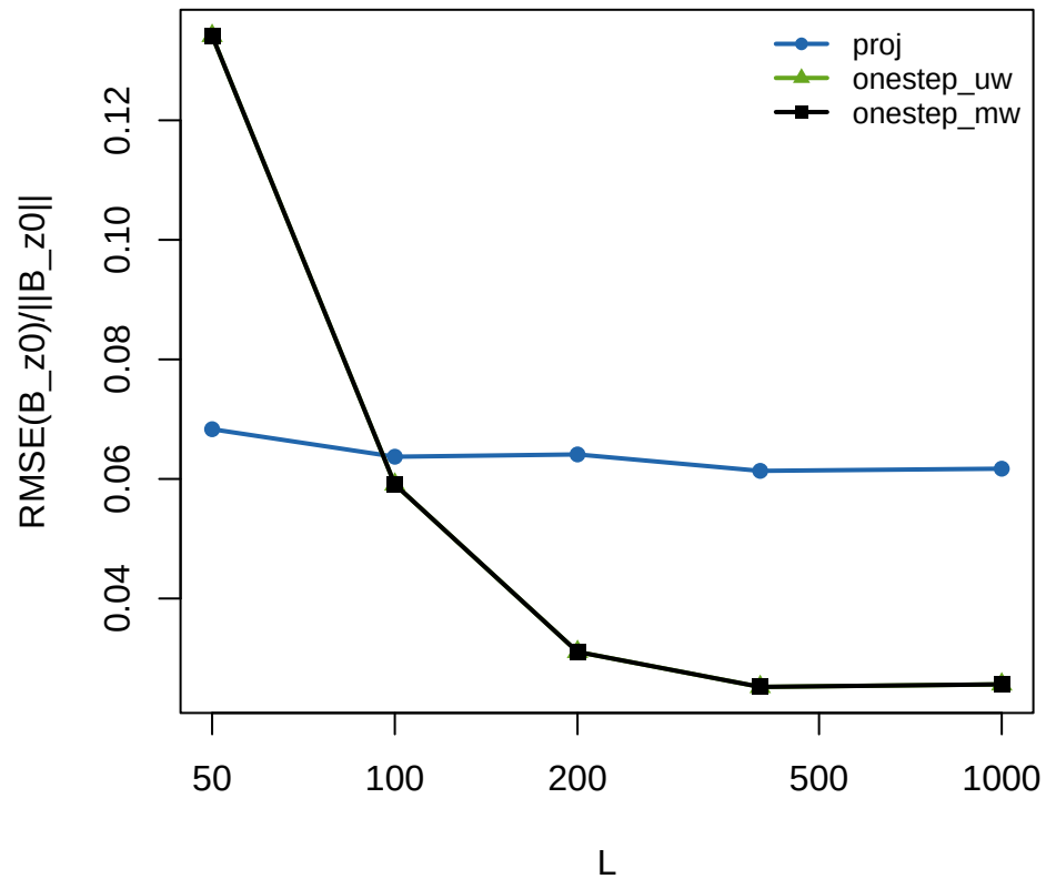
G5c: RMSE vs document length
