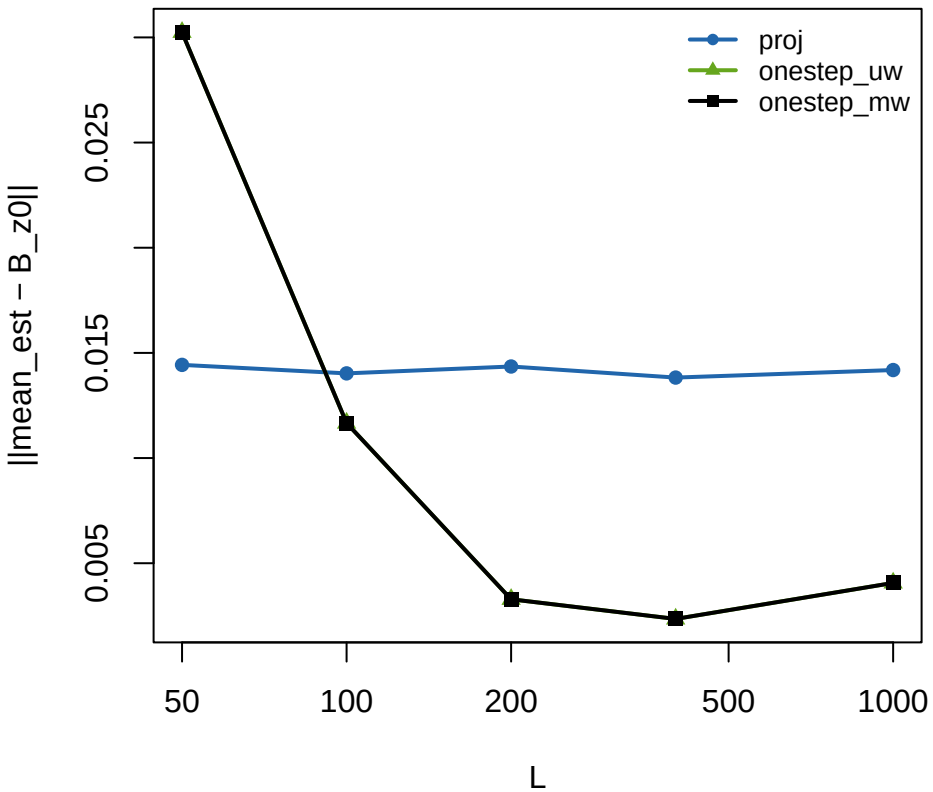
G5c: one-step bias vs document length
