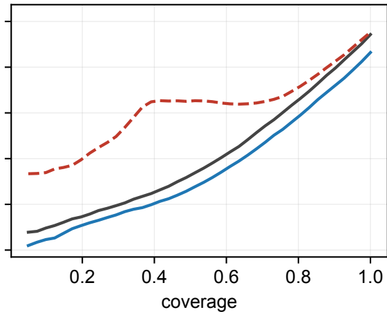
Qwen3.5-2B
