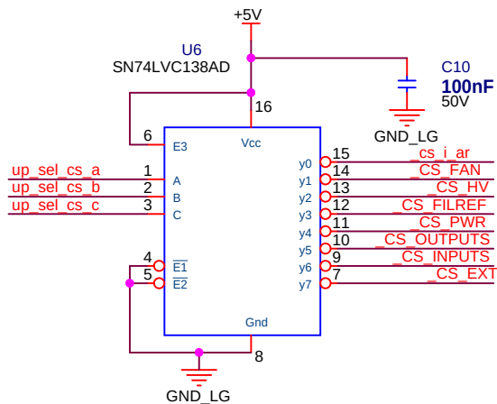
SPI CHIP SELECT DEMULTIPLEXER
