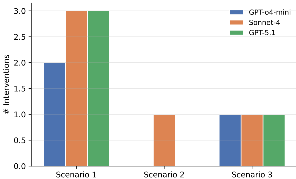
User Interventions per Scenario
