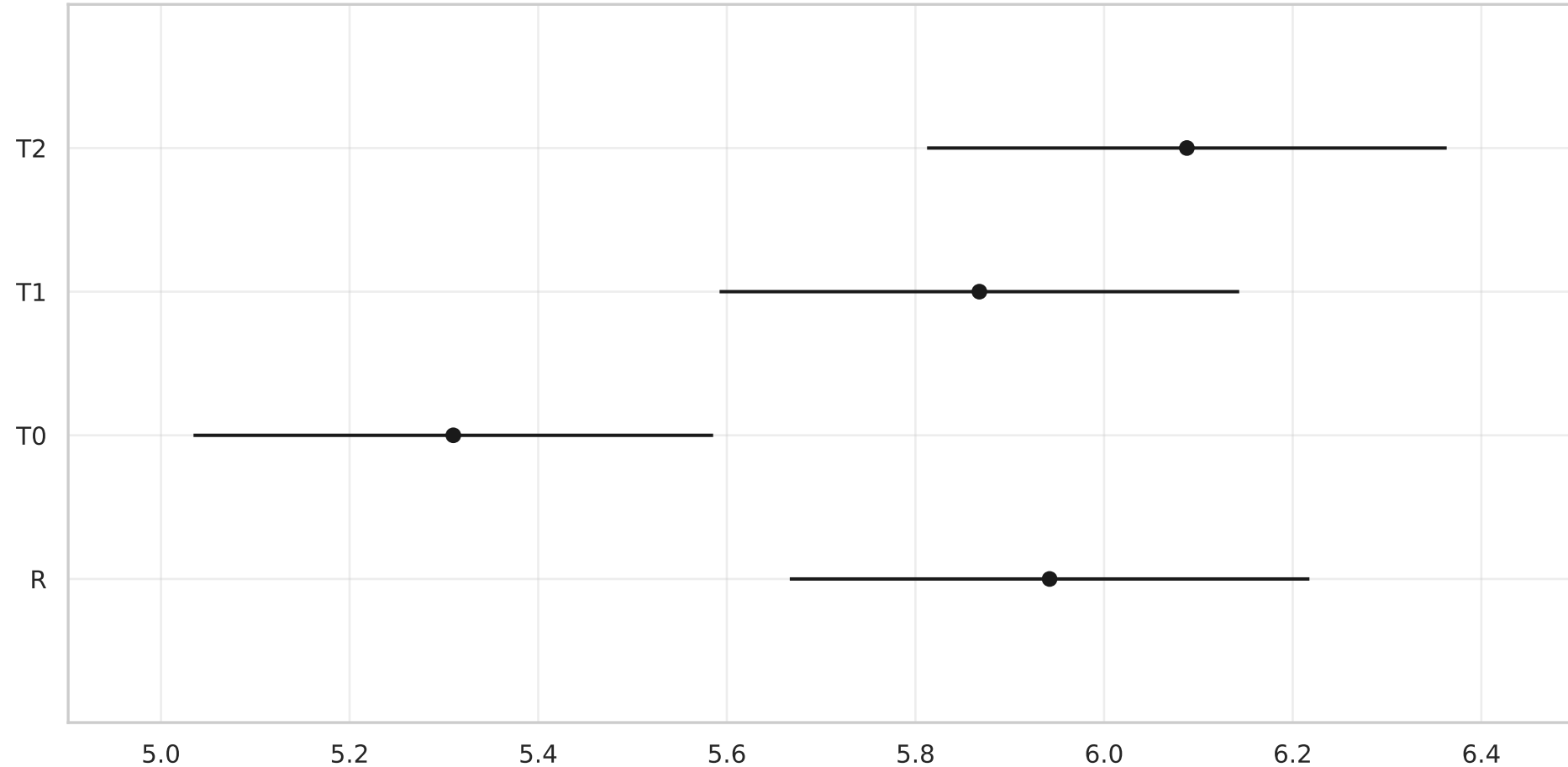
Multiple Comparisons Between All Pairs (Tukey)
