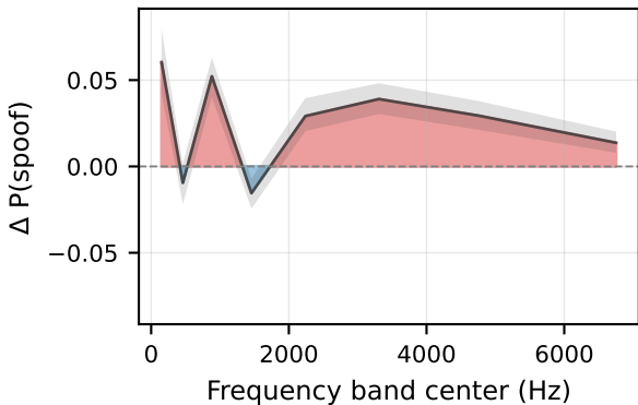
D_{ad} (adapted)
