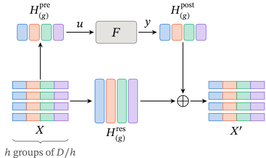
(b) Multi-head mHC, here with h = 4
