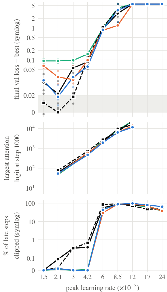
Without QK-norm: best mean 4.100
