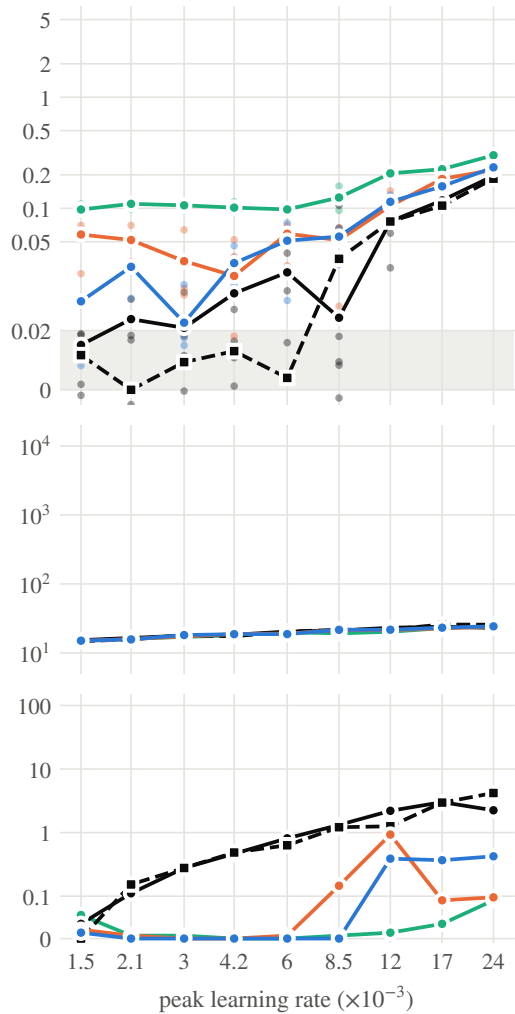
With QK-norm: best mean 4.059
