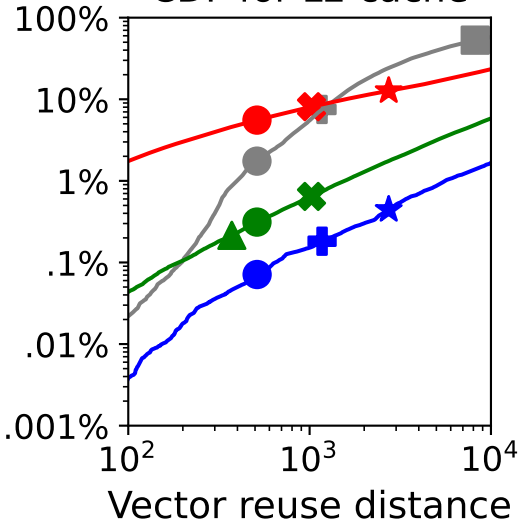
CDF for L2 cache
