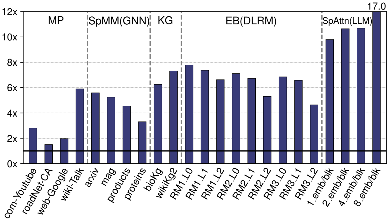
Speedup of DAE optimizations
