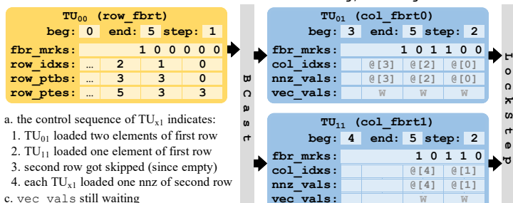
Time 3: first row has all elements outstanding, loading second row
