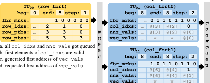
Time 4: starts to load dense-vector values (lookup operation)
