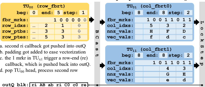
Time 6: all elements of the first row got queued into the outQ
