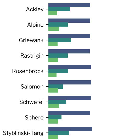
Execution Time Comparison (750D)
