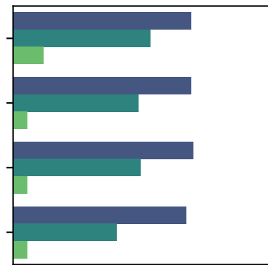
Dimension = 512
