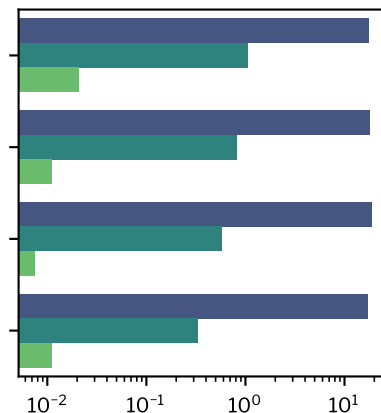
Dimension = 512
