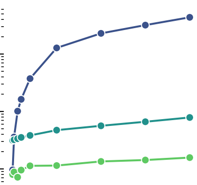
Sphere
