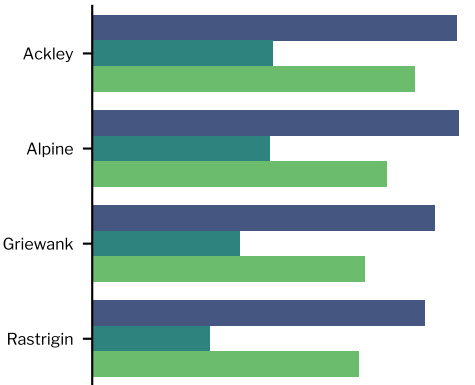
Dimension = 50
