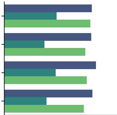
Dimension = 30
