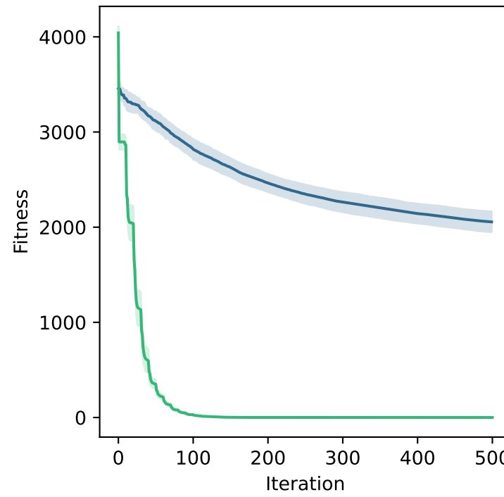
Sphere - 500D
