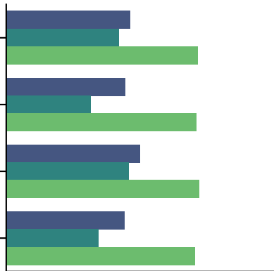
Dimension = 10
