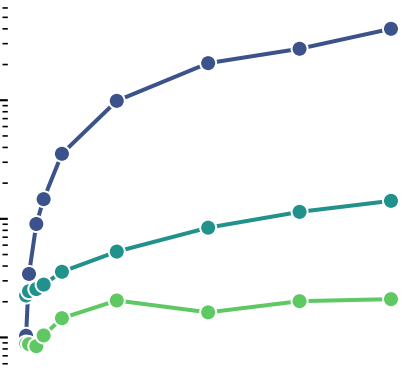
Rosenbrock
