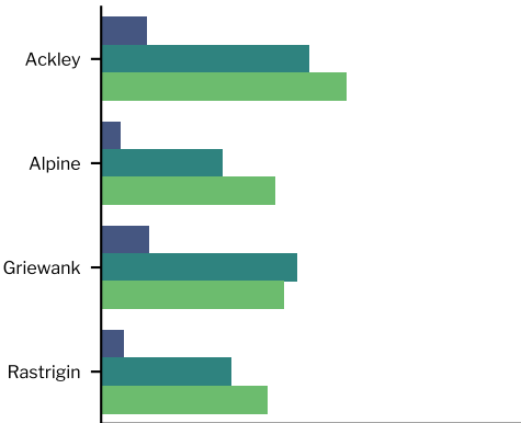
Dimension = 50
