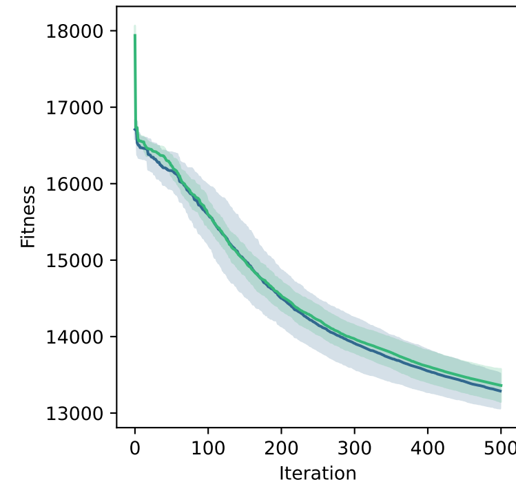
Rosenbrock - 1000D
