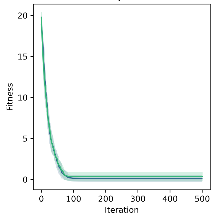
Rastrigin - 10D
