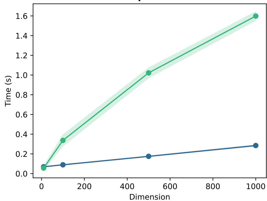
Sphere
