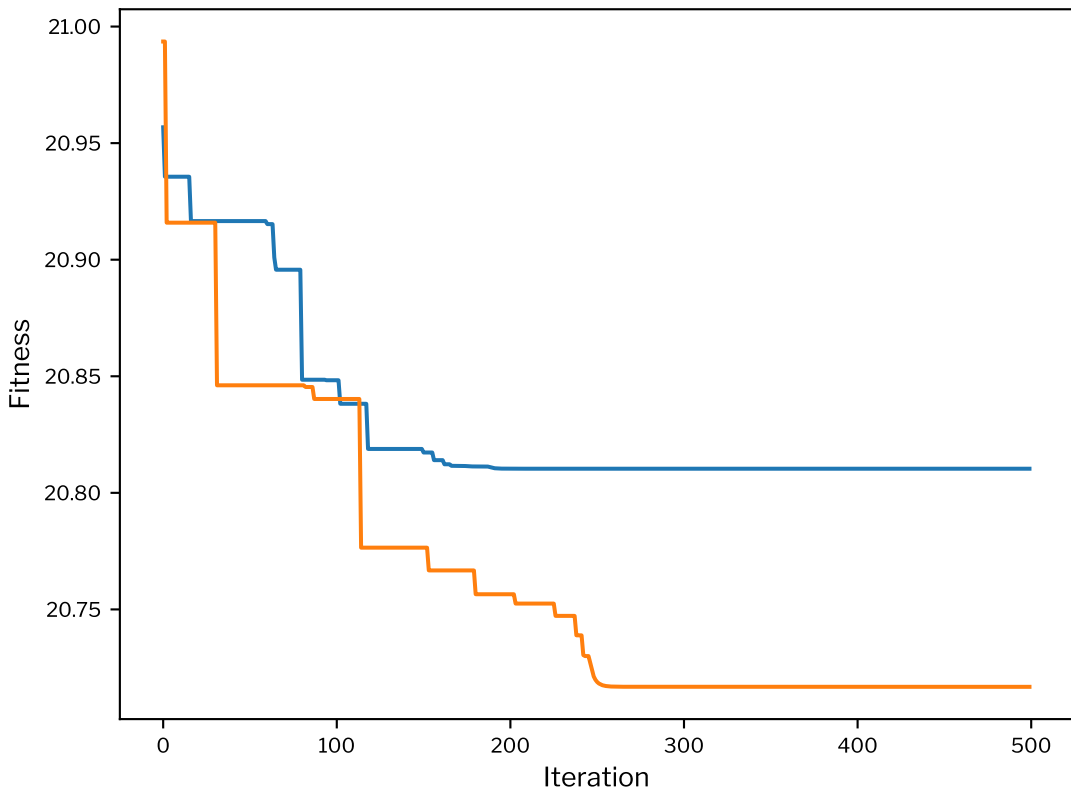
Convergence History
