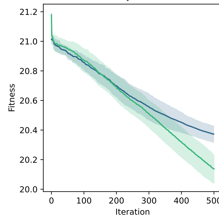
Rastrigin - 500D
