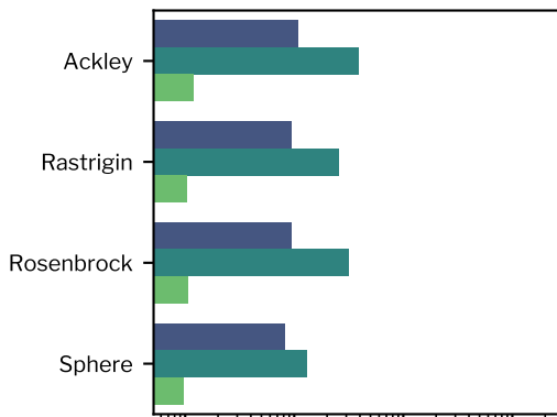
Dimension = 16
