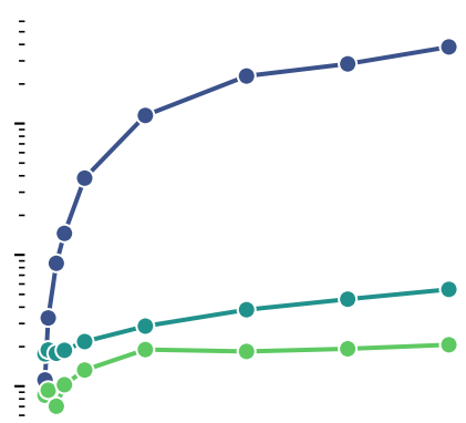
Styblinski-Tang
