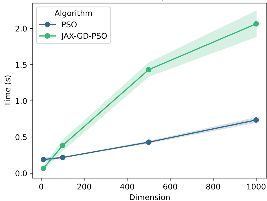
Rosenbrock
