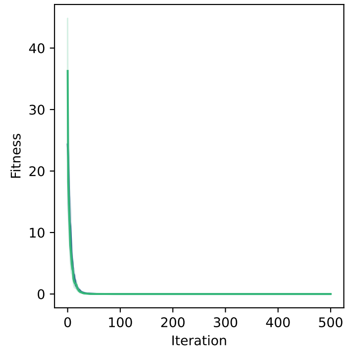
Sphere - 10D
