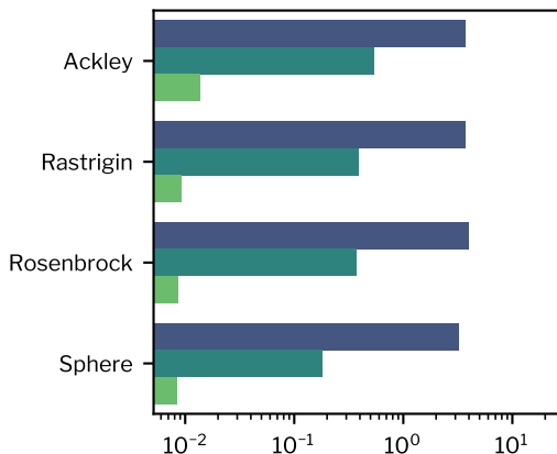
Dimension = 128
