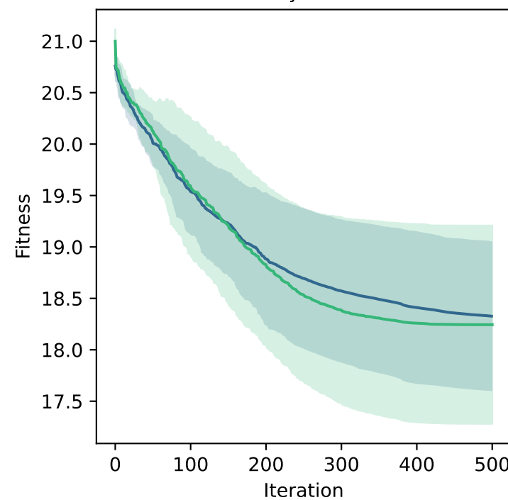
Rastrigin - 100D
