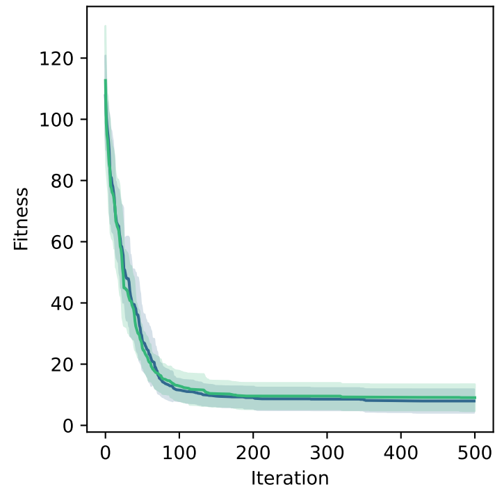
Rosenbrock - 10D
