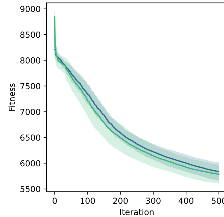
Rosenbrock - 500D
