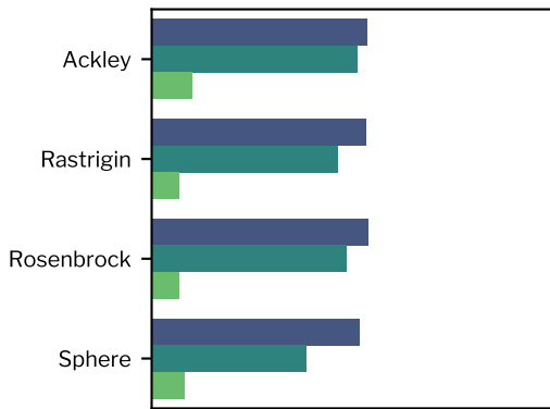
Dimension = 128
