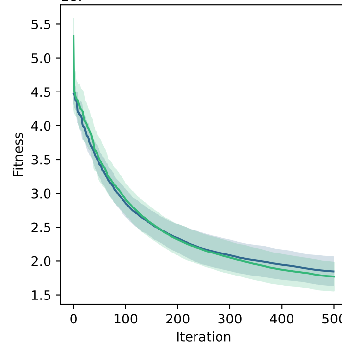
Sphere - 500D
