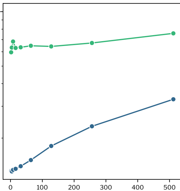
Sphere
