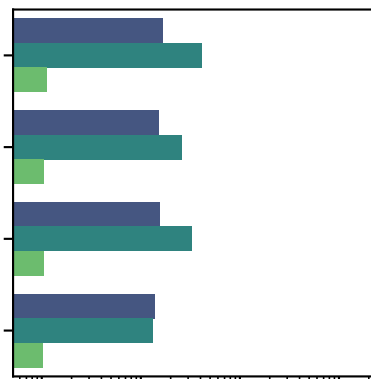
Dimension = 32
