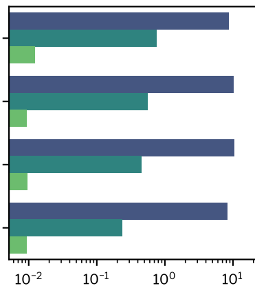
Dimension = 256
