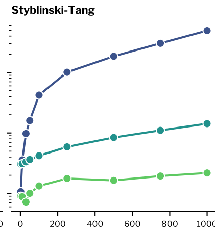
Styblinski-Tang
