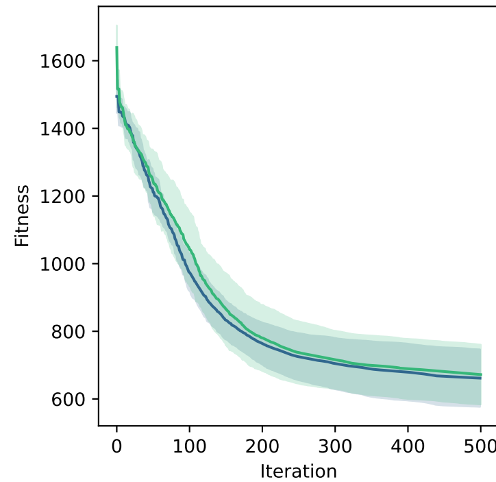
Rosenbrock - 100D
