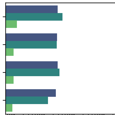
Dimension = 64
