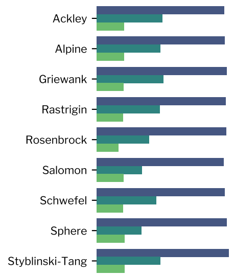
Execution Time Comparison (1000D)
