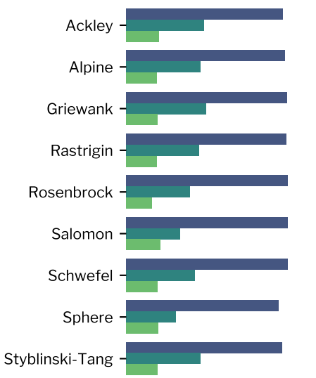
Execution Time Comparison (500D)
