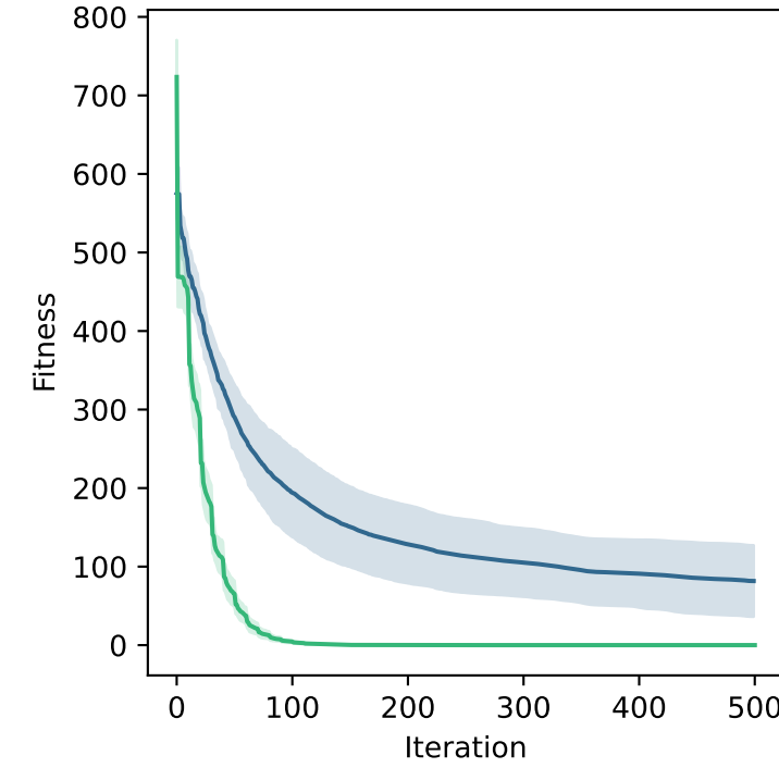
Sphere - 100D
