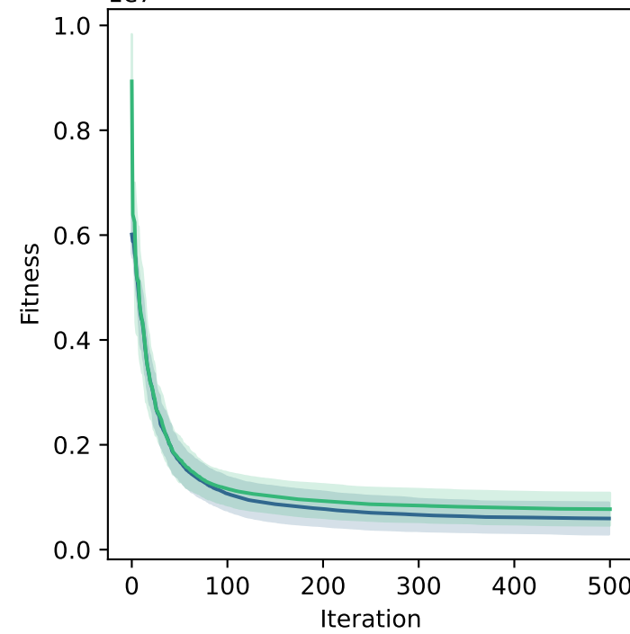
Sphere - 100D
