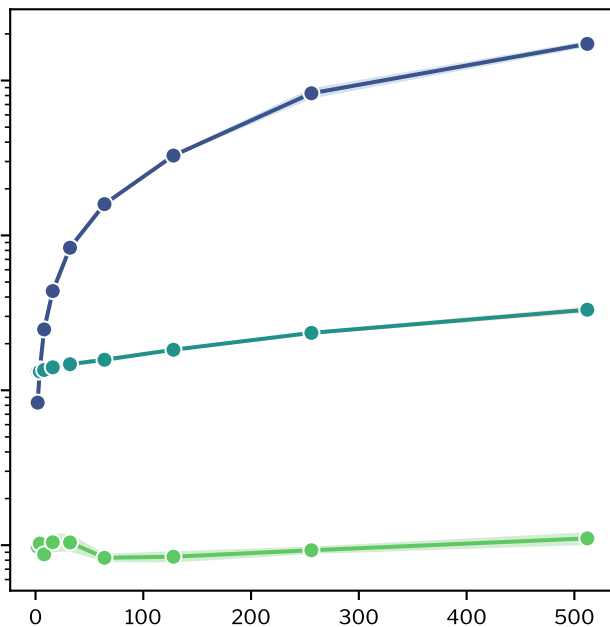
Sphere
