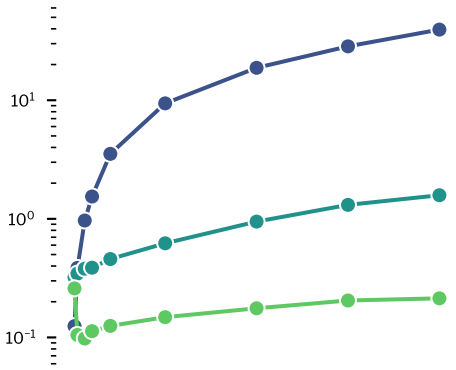
Rastrigin
