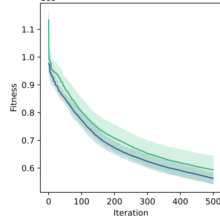
Sphere - 1000D
