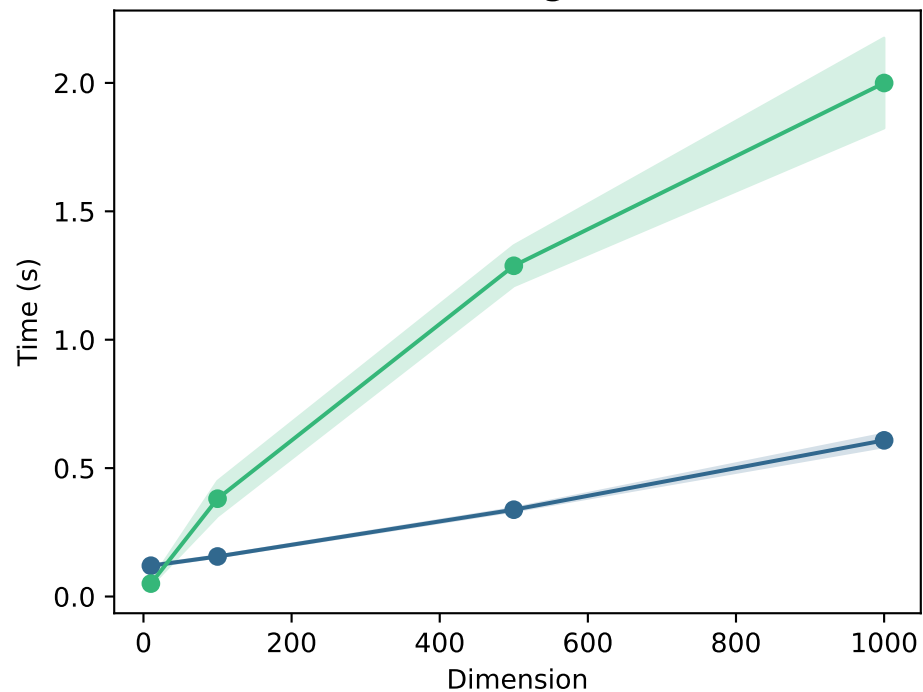
Sphere
