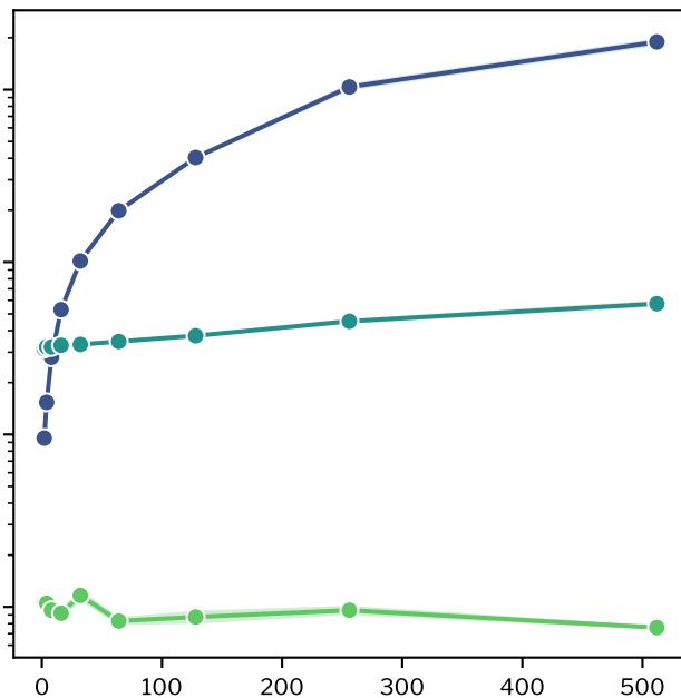
Rosenbrock
