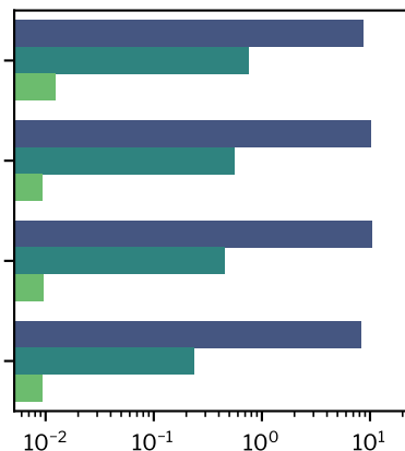
Dimension = 256
