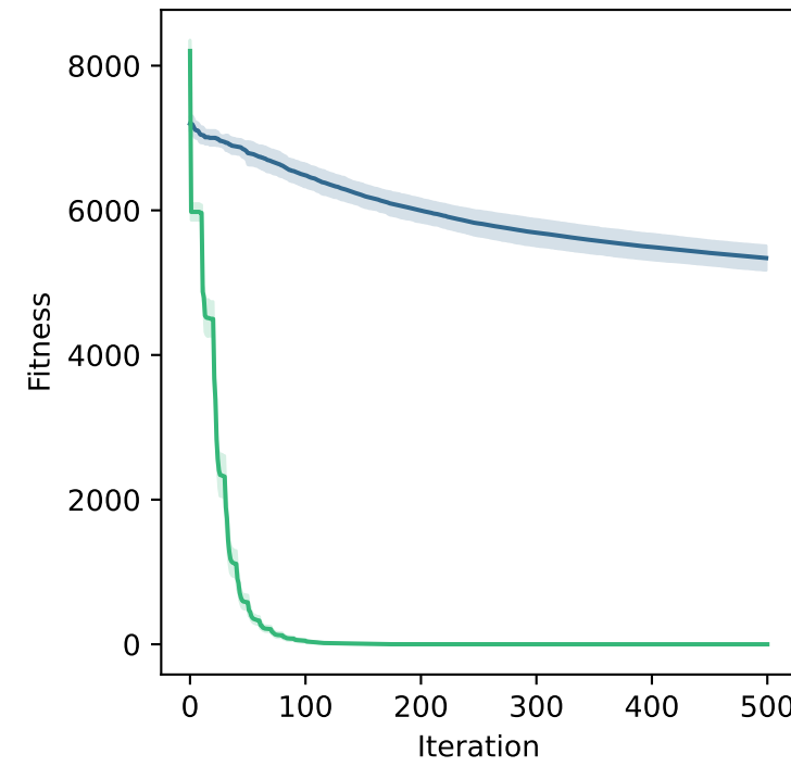
Sphere - 1000D
