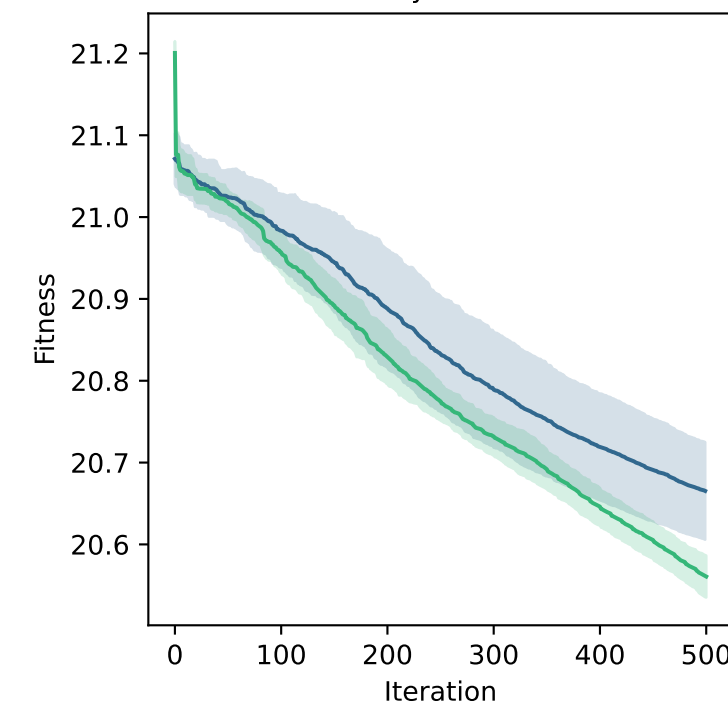
Rastrigin - 1000D
