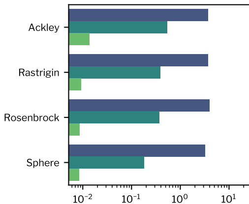
Dimension = 128
