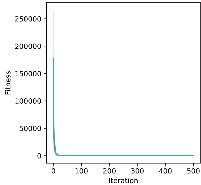
Sphere - 10D
