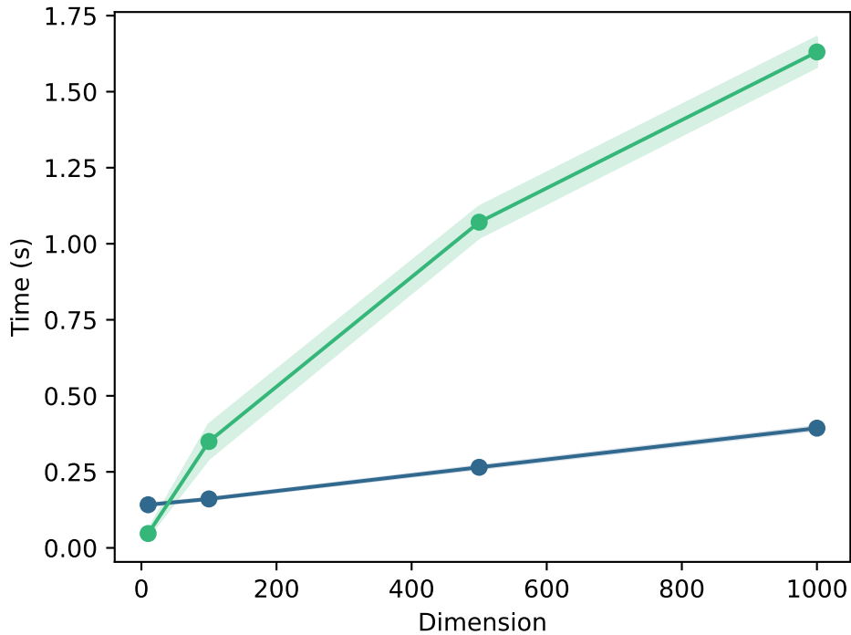
Rosenbrock
