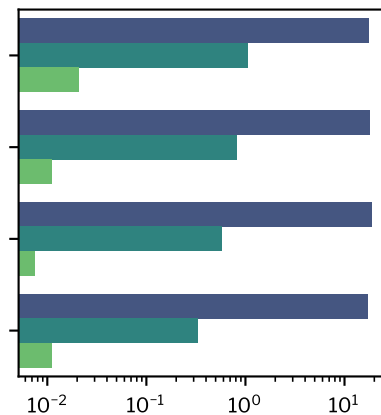
Dimension = 512
