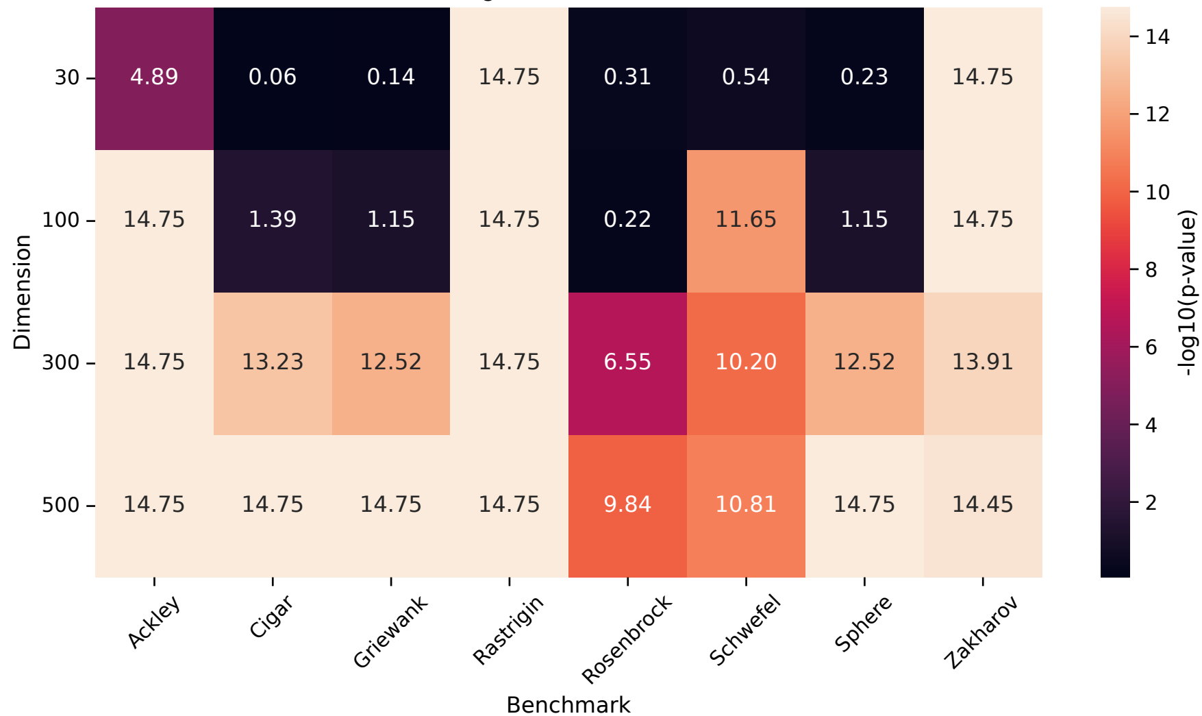
Statistical Significance DRS-PSO vs PSO)
