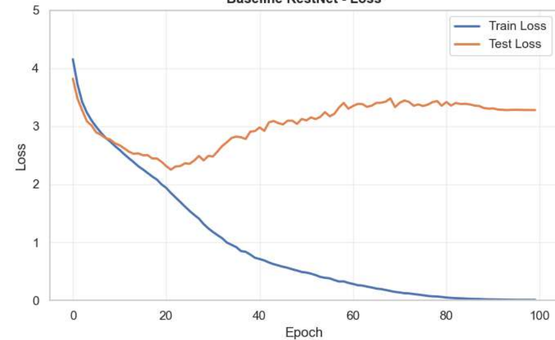
Baseline RestNet - Loss
