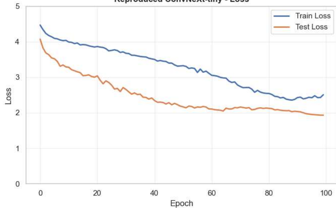
Reproduced ConvNeXt-tiny - Loss
