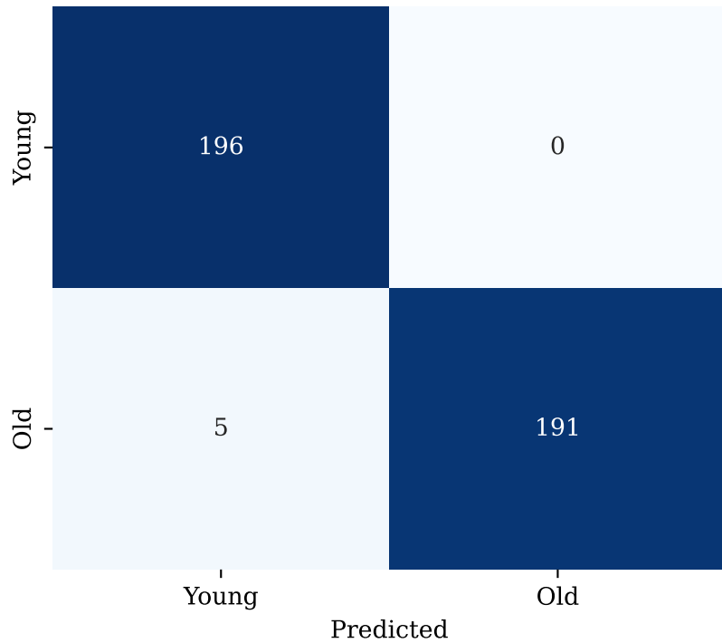
Confusion matrix — SVM (RBF) (SOC=3)
