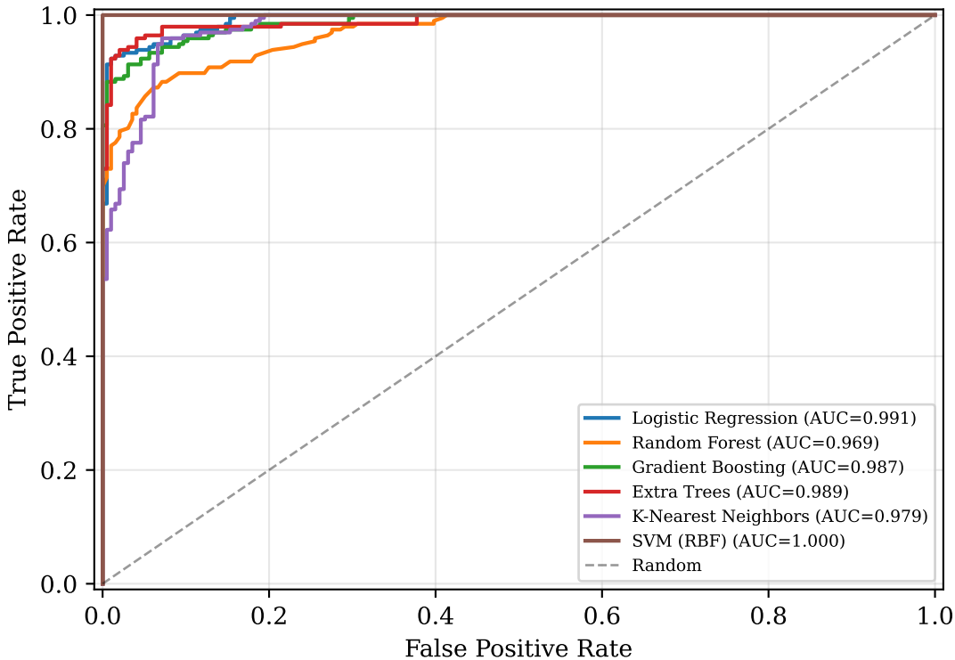
Task 2 — ROC curves (SOC=3)
