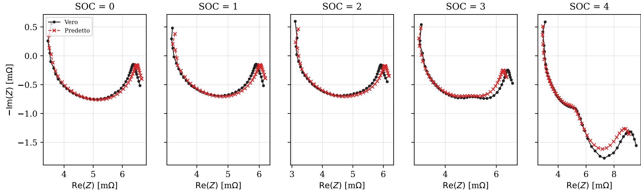
Task 1 — Vero vs Predetto (Aging=2, T=22.5°C, modello: K-Nearest Neighbors)
