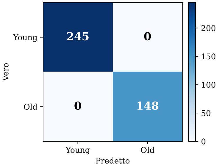
Confusion matrix — SVM (RBF) (SOC=3)
