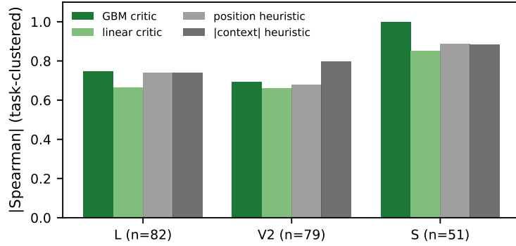
Figure 6: F4 — Critics vs. trivial heuristics per stratum (task-clustered |\text{Spearman}| ). The critic never beats the best heuristic; C_H is structured by position and context size.
