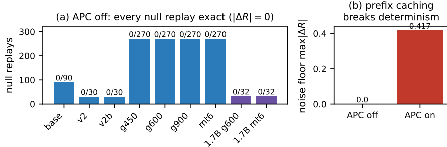
Figure 1: F1 — Measured noise floor. (a) Dedicated null-replay runs (Qwen3-4B blue, Qwen3-1.7B purple); together with nulls attached to interaction runs and the Qwen3-8B replication, all 2,739 null replays are exact, floor = 0.0. (b) With vLLM automatic prefix caching on, the floor rises to 0.417 (7/270 inexact): greedy determinism breaks silently.
