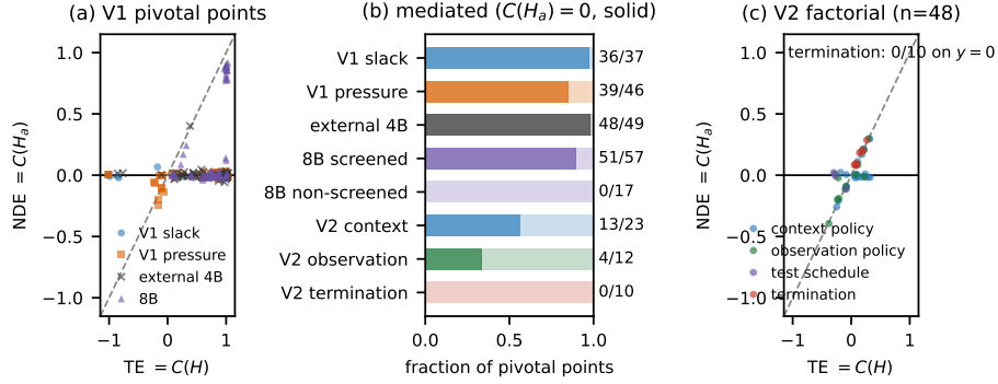
Figure 2: Total vs. direct harness effect (pre-reg 40 and 42 rows). (a) Harness-pivotal V1 points: designed pool by regime, external 4B (crosses) and 8B (triangles); mediated points sit on C_{Ha} = 0 , the 8B’s screening breaks near the diagonal C_{Ha} = C_H . (b) Fraction of pivotal points with C_{Ha} = 0 per population (solid), k/n annotated. (c) V2, 48 points by type: termination lies on the diagonal (no mediation, 0/10). Jitter \sigma = 0.015 .
