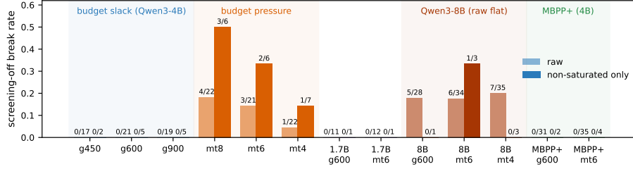
Figure 3: F3 — Screening-off is regime-dependent, and the regime contrast is model-dependent. Break rate of C_{HM} = C_M per configuration, raw and conditioned on non-saturated points. Slack: 0/57 raw (0/12 non-saturated). Pressure: 8/65 raw (6/19 non-saturated, p = 0.037 ). Qwen3-1.7B (purple) replicates slack; its pressure null is explained by saturation (only 1 non-saturated point). Qwen3-8B (red) breaks raw screening at a flat rate across regimes (5/28, 6/34, 7/35) — the shield inversion of §7. MBPP+ (green, Qwen3-4B) replicates screening unconditionally (0/66).
