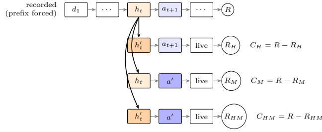
Figure 1: The three-arm replay at one interaction point. The recorded prefix is forced up to the harness decision h_t ; each arm changes exactly one thing (the harness decision, the model action, or both) and runs live from there. Interaction is I = C_{HM} - C_H - C_M ; screening-off is the event C_{HM} = C_M : the harness flip adds nothing beyond the model’s alternative.
