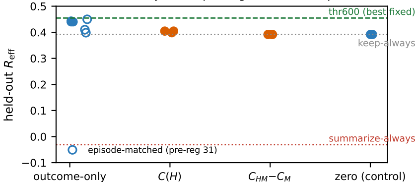
Act 4 (sane objective, pre-reg 27): 3 seeds per arm
