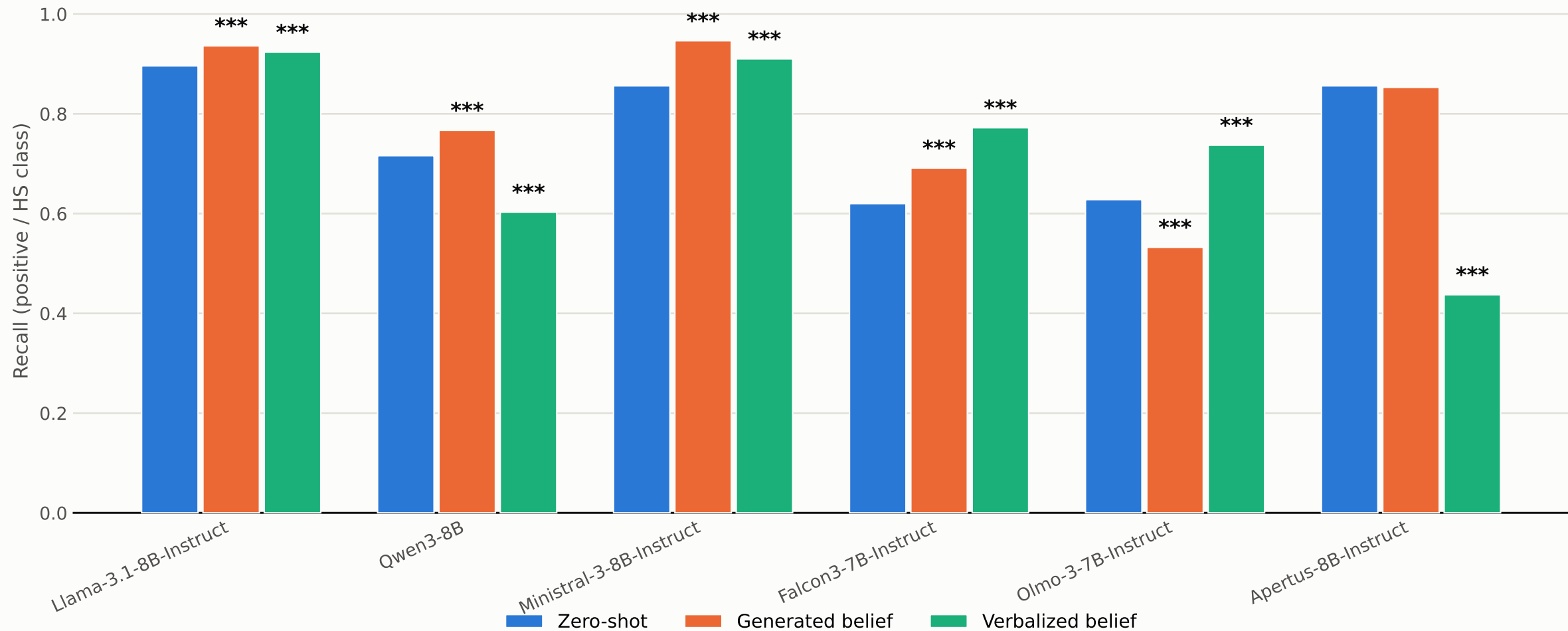
Hate-speech classification recall by model and condition
