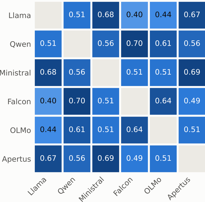
Zero-shot
