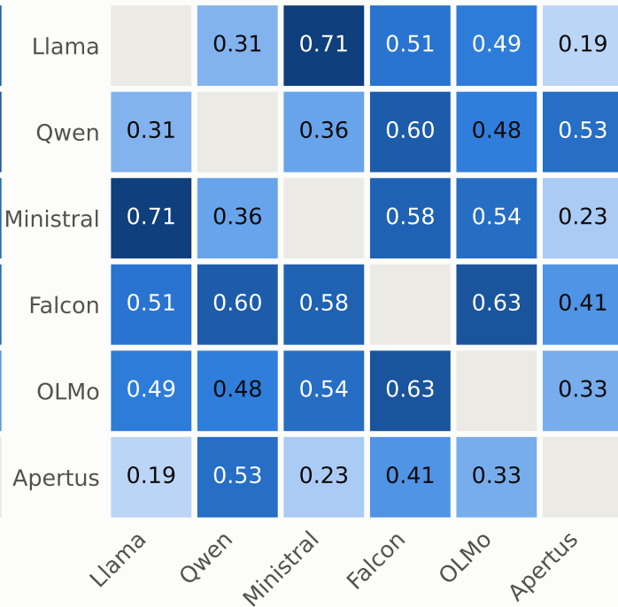
Verbalized belief
