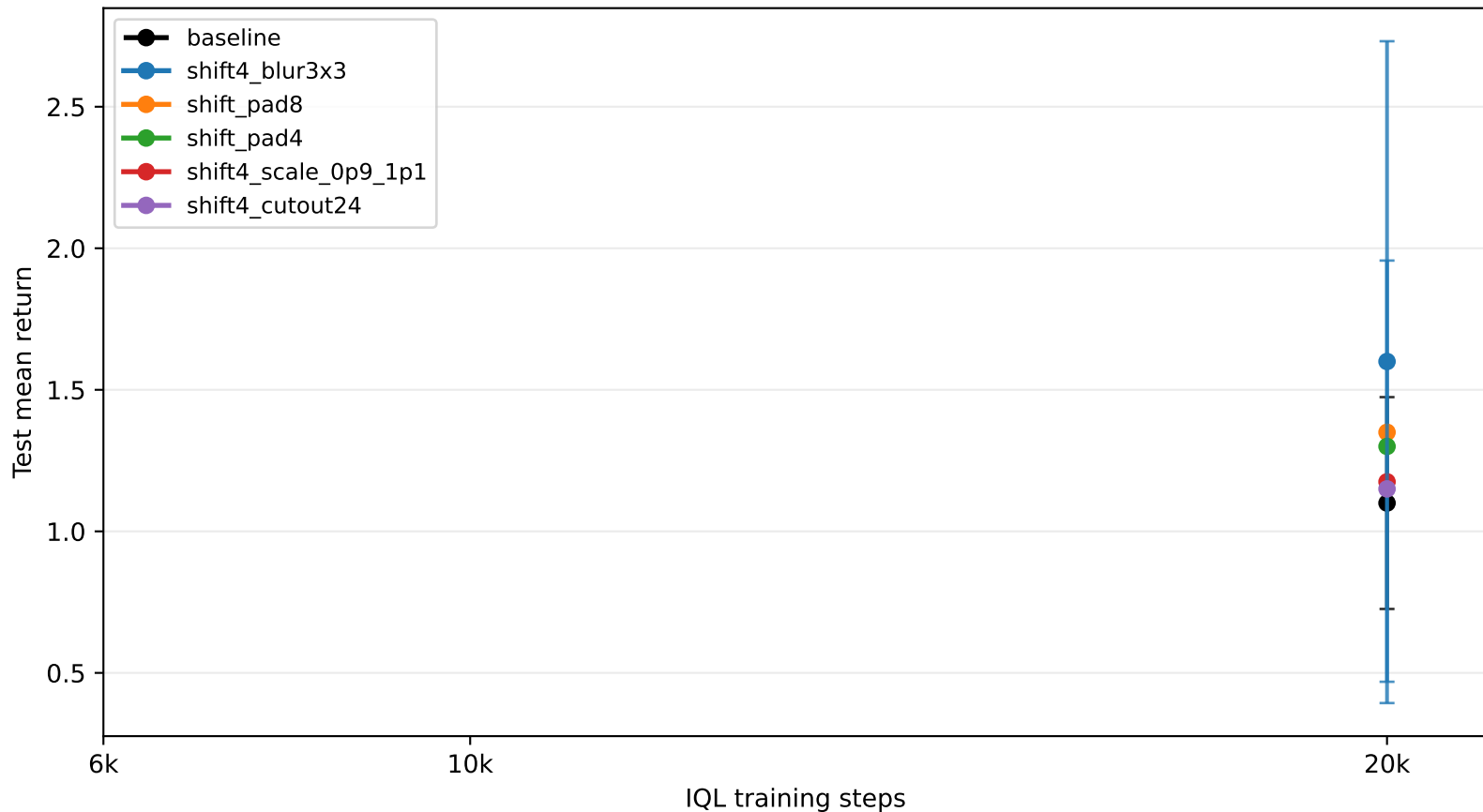
IQL: top augmentations vs steps (rank@20000)
