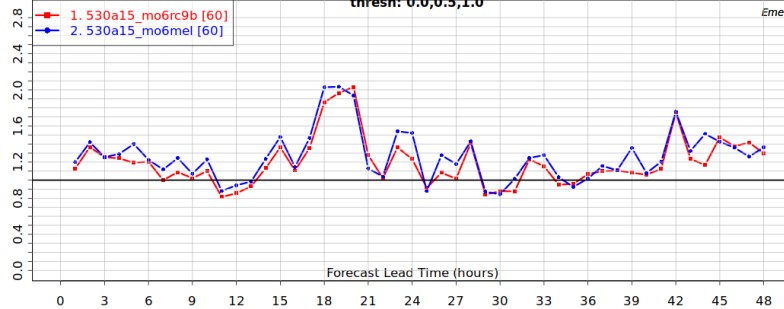
ENCY BIAS INDEX OF 1-HOUR FREEZ. RAIN/DRIZZLE VS METAR PRECIP. TYPE (with precip condition) 2022-01-01 @ 2022-03-01 PR>=0.1 ade metar speci North America plus thresh: 0.0,0.5,1.0
