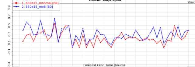
1LE THREAT SCORE OF 1-HOUR FREEZ. RAIN/DRIZZLE VS METAR PRECIP. TYPE (with precip condition) 2022-01-01 @ 2022-03-10 PR>=2 ade metar speci North America plus thresh: 0.0,0.5,1.0
