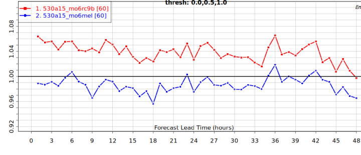
FREQUENCY BIAS INDEX OF 1-HOUR SNOW VS METAR PRECIP. TYPE (with precip condition) 2022-01-01 @ 2022-03-01 PR>=0.1 ade metar speci North America plus thresh: 0.0,0.5,1.0
