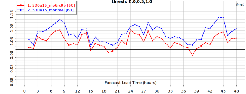
EQUENCY BIAS INDEX OF 1-HOUR RAIN/DRIZZLE VS METAR PRECIP. TYPE (with precip condition) 2022-01-01 @ 2022-03-01 PR>=1 ade metar speci North America plus thresh: 0.0,0.5,1.0
