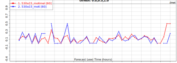
UTABLE THREAT SCORE OF 1-HOUR ICE PELLET VS METAR PRECIP. TYPE (with precip condition) 2022-01-01 @ 2022-03-10 PR>=2 ade metar speci North America plus thresh: 0.0,0.5,1.0
