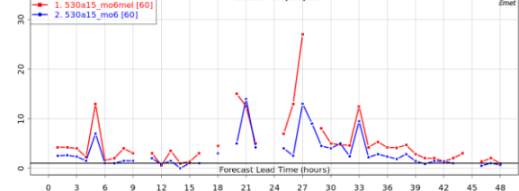
REQUENCY BIAS INDEX OF 1-HOUR ICE PELLET VS METAR PRECIP. TYPE (with precip condition) 2022-01-01 @ 2022-03-10 PR>=2 ade metar speci North America plus thresh: 0.0,0.5,1.0
