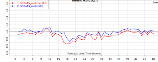
FREQUENCY BIAS INDEX OF 1-HOUR SNOW VS METAR PRECIP. TYPE (with precip condition) 2022-01-01 @ 2022-03-10 PR>=2 ade metar speci North America plus thresh: 0.0,0.5,1.0
