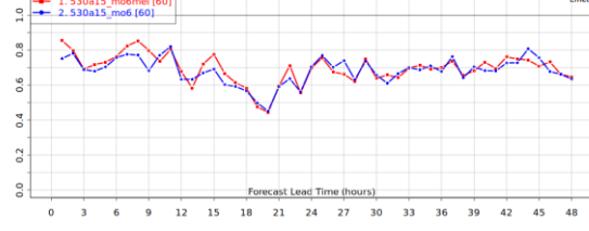
EQUITABLE THREAT SCORE OF 1-HOUR SNOW VS METAR PRECIP. TYPE (with precip condition) 2022-01-01 @ 2022-03-10 PR>=2 ade metar speci North America plus thresh: 0.0,0.5,1.0
