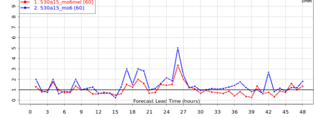
ENCY BIAS INDEX OF 1-HOUR FREEZ. RAIN/DRIZZLE VS METAR PRECIP. TYPE (with precip condition) 2022-01-01 @ 2°C PR>=2 ade metar speci North America plus thresh: 0.0,0.5,1.0
