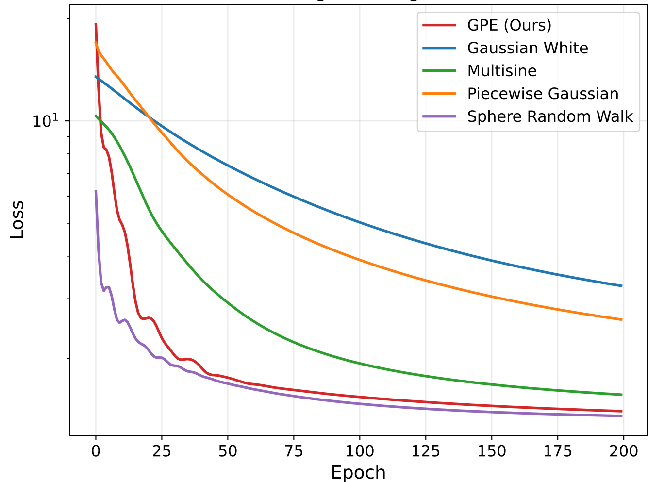
Training Convergence
