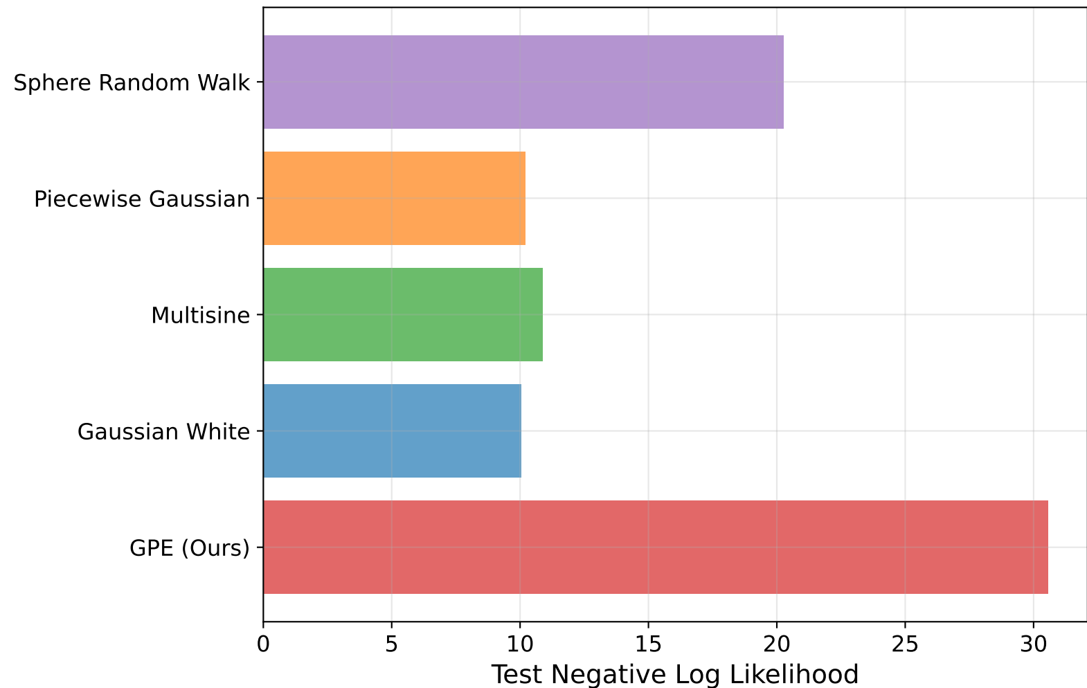
Generalization Performance
