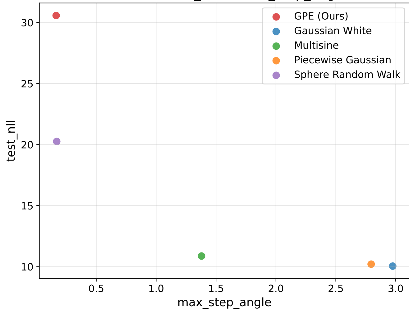
Trade-off: test_nll vs max_step_angle
